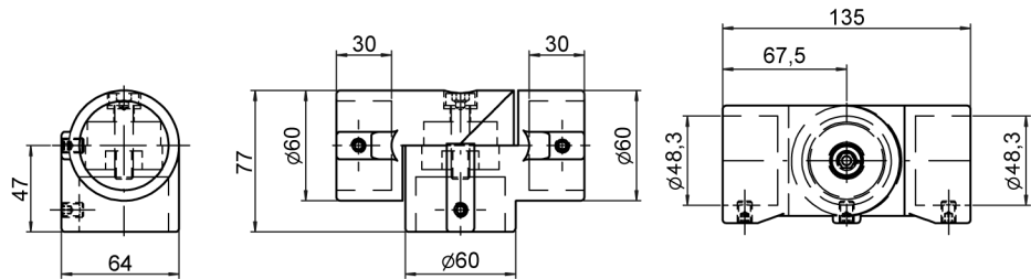
T-Gelenkverbinder, 1-schalig T-joint connector, 1-shell
