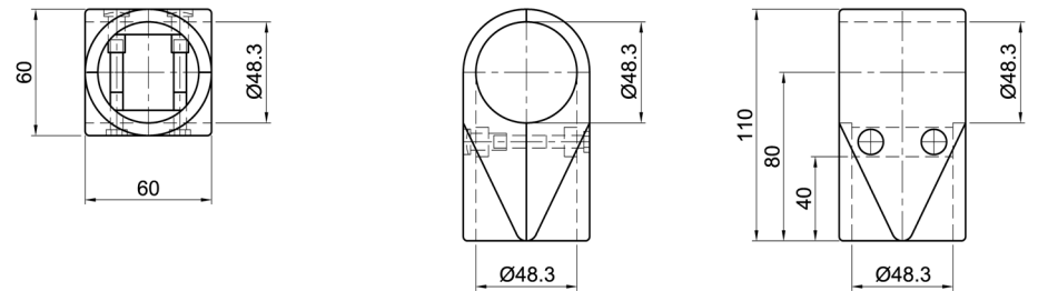
T-Gelenkverbinder, 1-schalig T-joint connector, 1-shell
