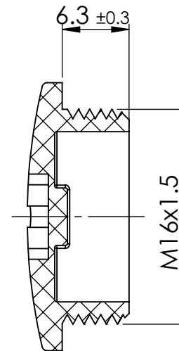
SECTION Y-Y
