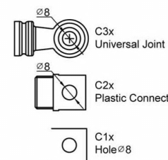
Front Connector
